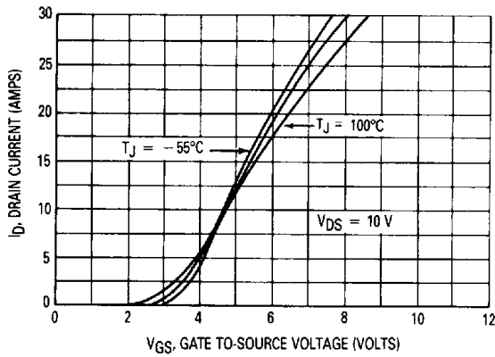
Figure 3. Transfer Characteristics
