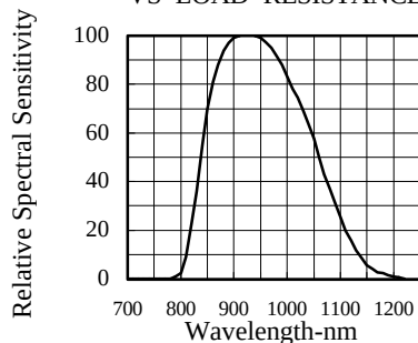
FIG.5 RELATIVE SPECTRAL SENSITIVITY VS. WAVELENGTH
