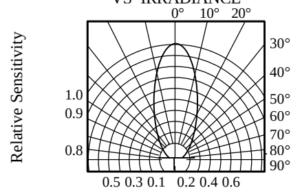
FIG.6 SENSITIVITY DIAGRAM
