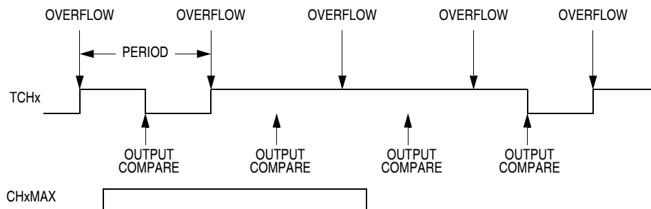
Figure 17-12. CHxMAX Latency
