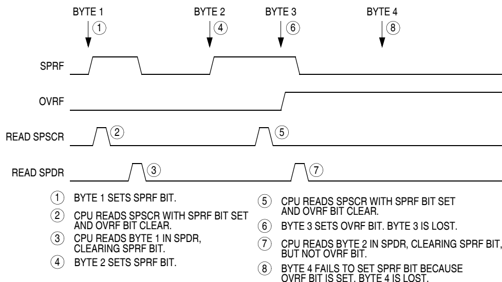
Figure 14-9. Missed Read of Overflow Condition
