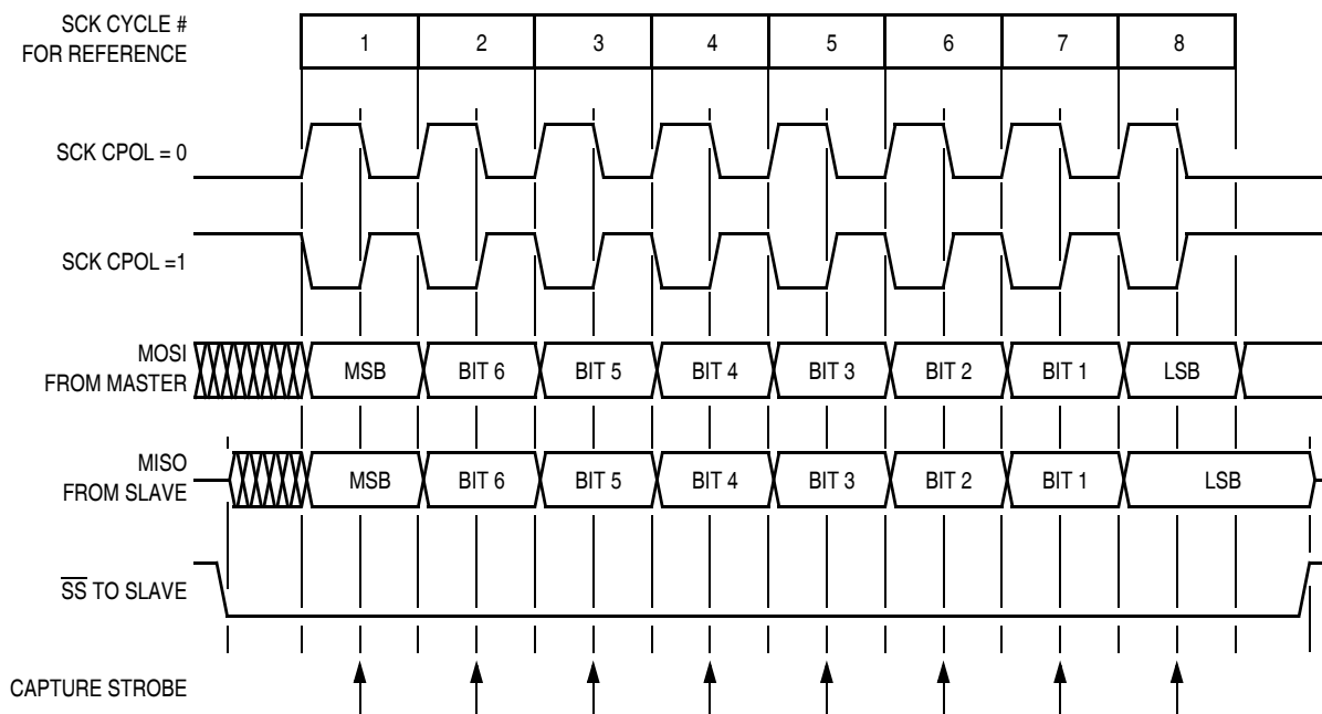
Figure 14-7. Transmission Format (CPHA = 1)
