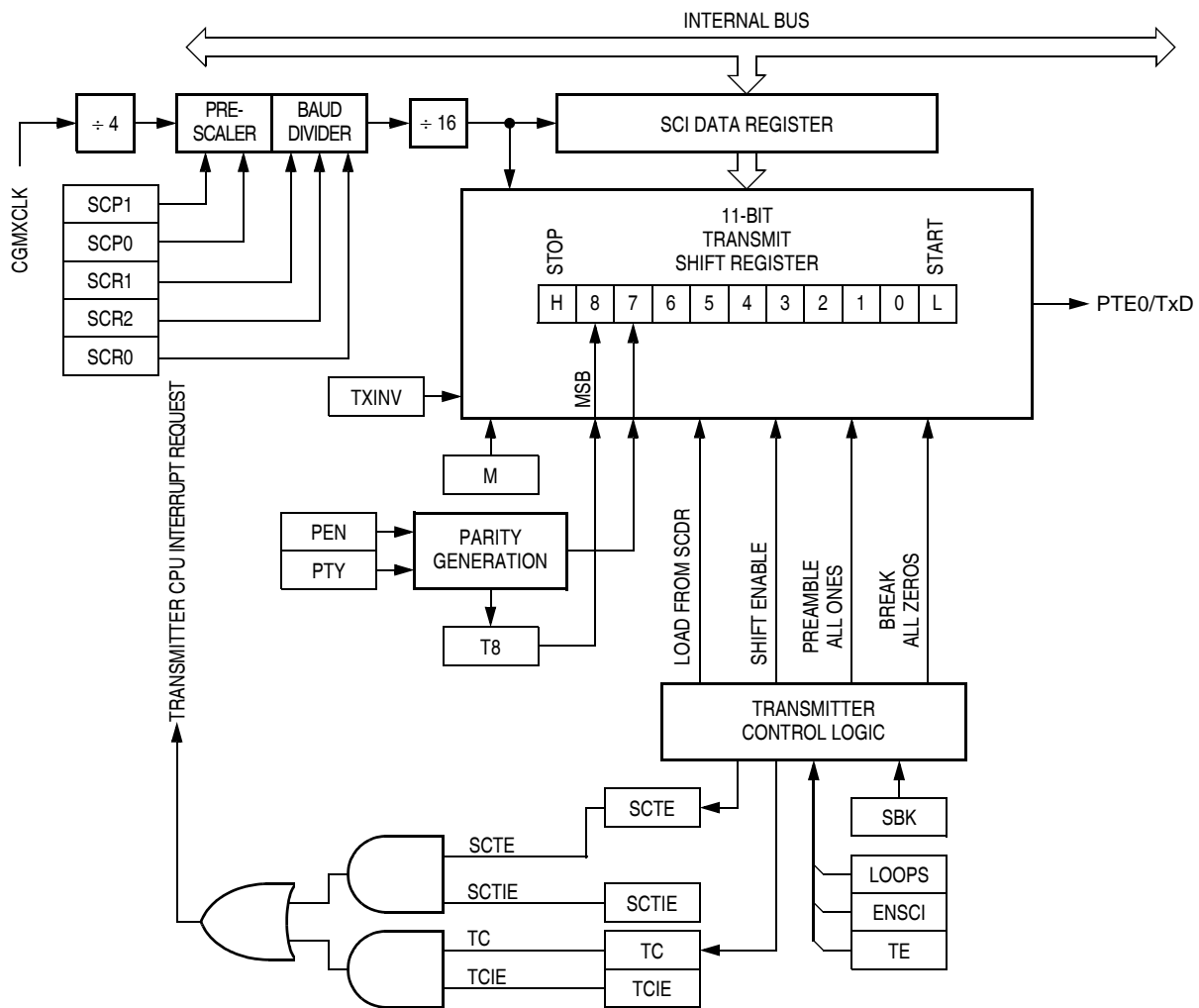
Figure 12-5. SCI Transmitter
