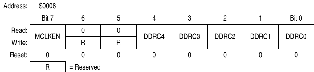
Figure 11-9. Data Direction Register C (DDRC)
