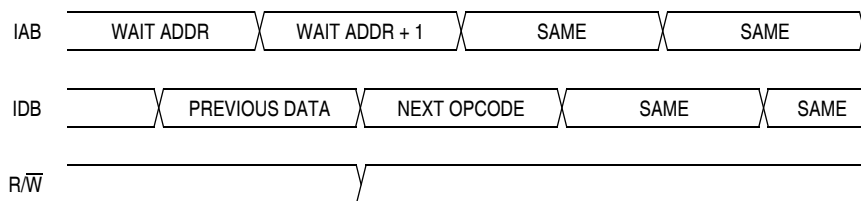
Figure 13-13. Wait Mode Entry Timing
