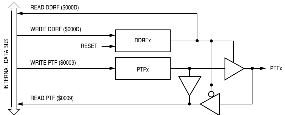
Figure 11-19. Port F I/O Circuit
