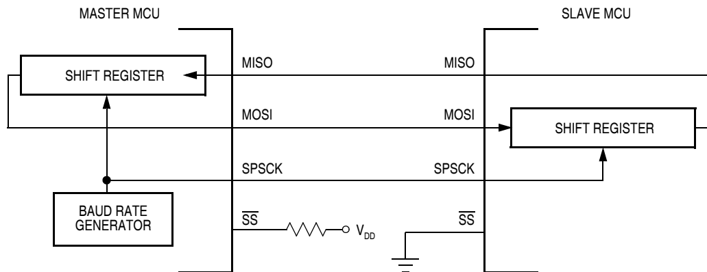
Figure 14-4. Full-Duplex Master-Slave Connections
