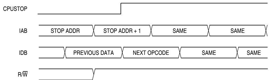
Figure 13-16. Stop Mode Entry Timing
