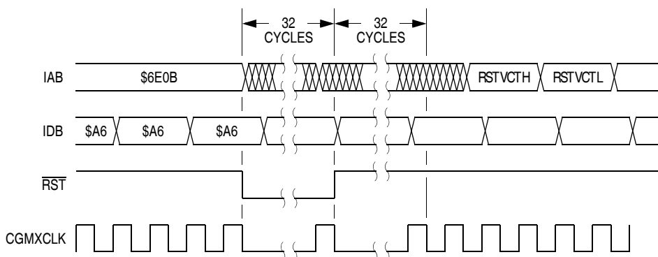
Figure 13-15. Wait Recovery from Internal Reset
