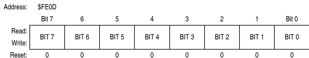
Figure 16-5. Break Address Register (BRKL)
