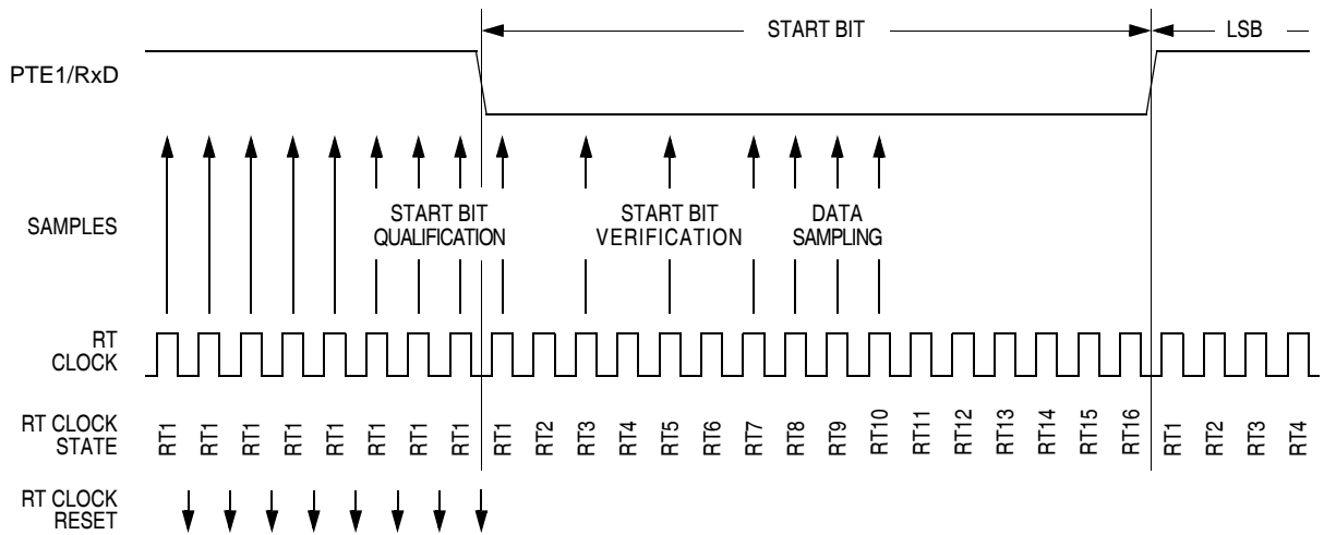
Figure 12-7. Receiver Data Sampling
