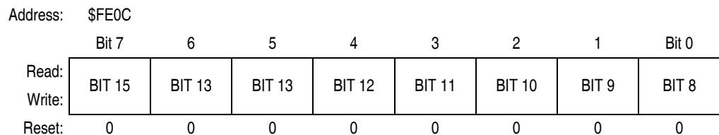
Figure 16-4. Break Address Register (BRKH)
