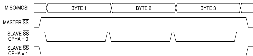
Figure 14-6. CPHA/\overline{SS} Timing
