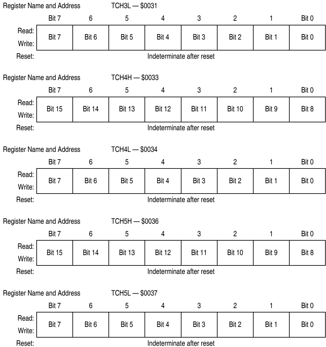
Figure 15-10. TIM Channel Registers (TCH0H/L–TCH3H/L) (Sheet 2 of 2)
