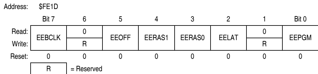
Figure 2-3. EEPROM Control Register (EECR)
