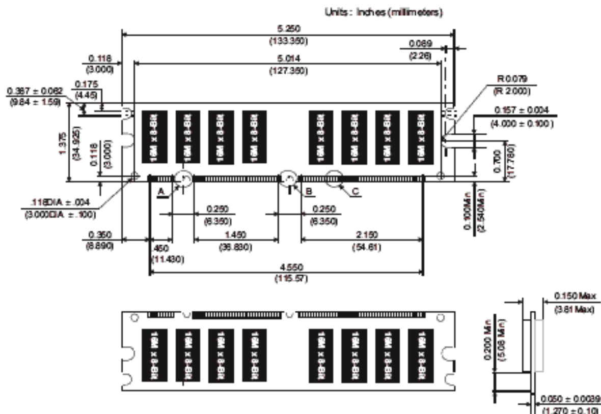
Figure 1: KVR100X64C2/256 168-Pin SDRAM Module
