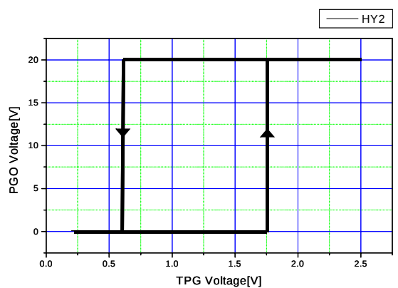
Figure 12. Hysteresis Voltage 2
