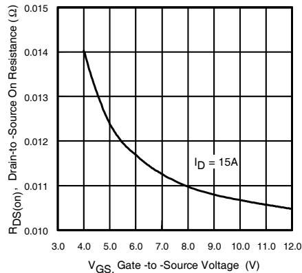
Figure 10. Typical R_{DS(on)} vs. Gate-to-Source Voltage
