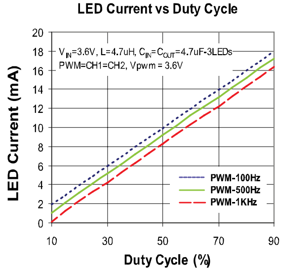
Figure 12. PWM Dimming
