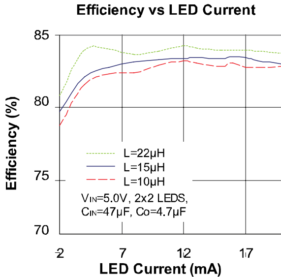
Figure 11. Peak power efficiency
