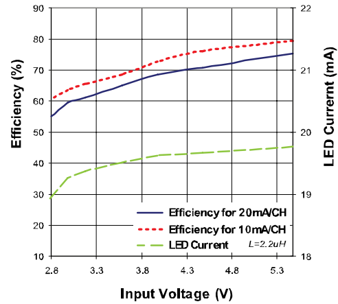
Figure 25. FAN5608 efficiency with twelve LEDs
