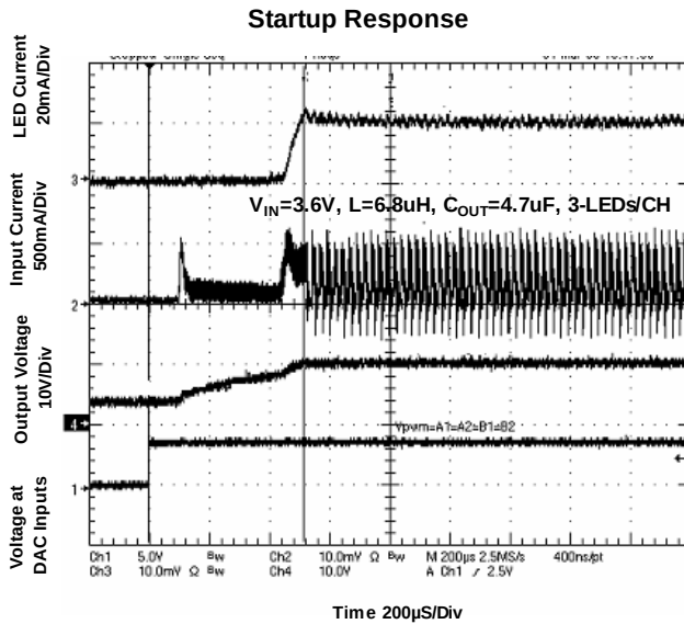
Figure 13. Startup Response
