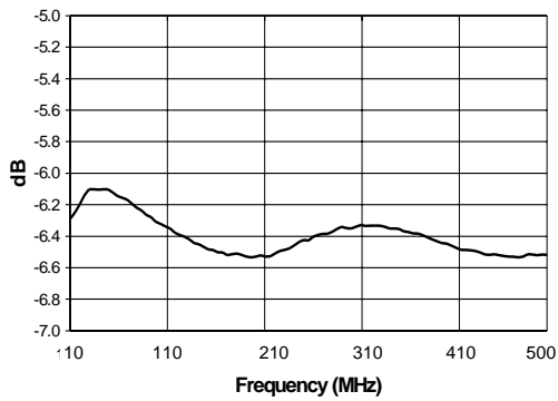
Conversion Loss
