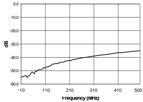
L-R Isolation
