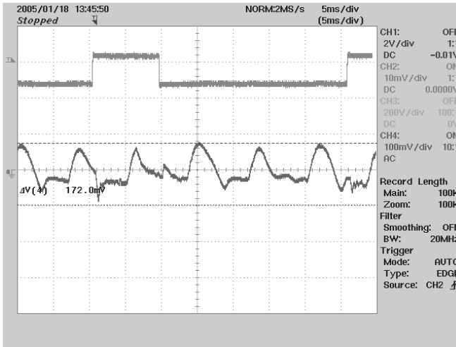
Figure 14 – Transient Response, 120 VAC, 75-100-75% Load Step. Top: Load Current, 0.5 A/div. Bottom: Output Voltage 100 mV, 5msec / div.
