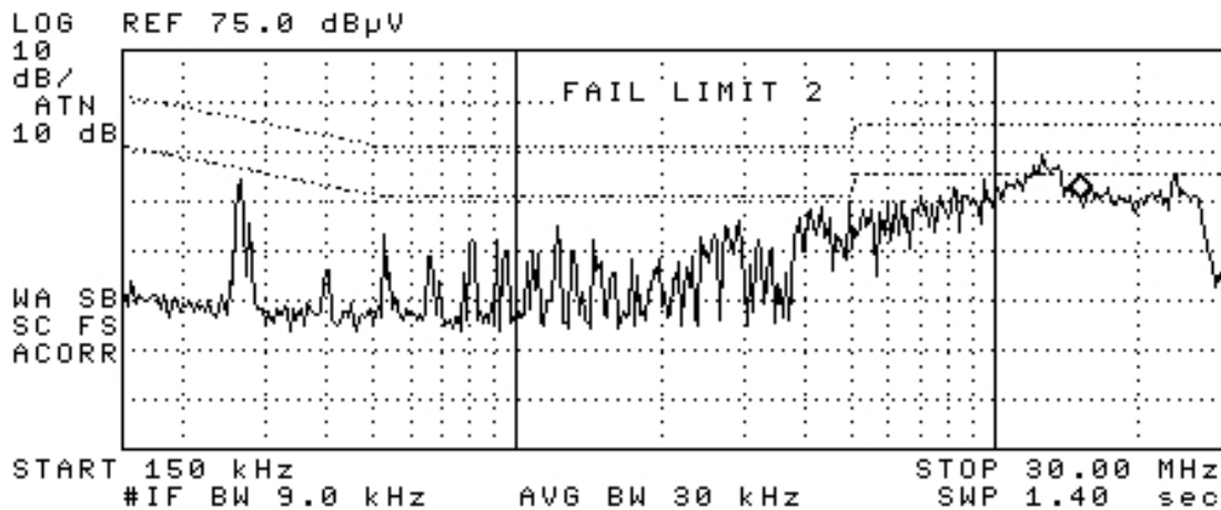
Figure 22 – Conducted EMI (Neutral), Maximum Load, 120 VAC, 60 Hz, and EN55022 B Limits
