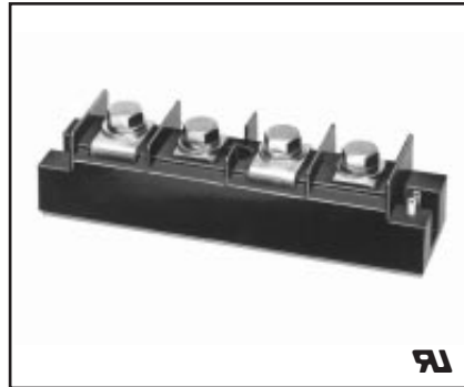
CM530813 Dual SCR POW-R-BLOK™ Modules 130 Amperes/800 Volts
