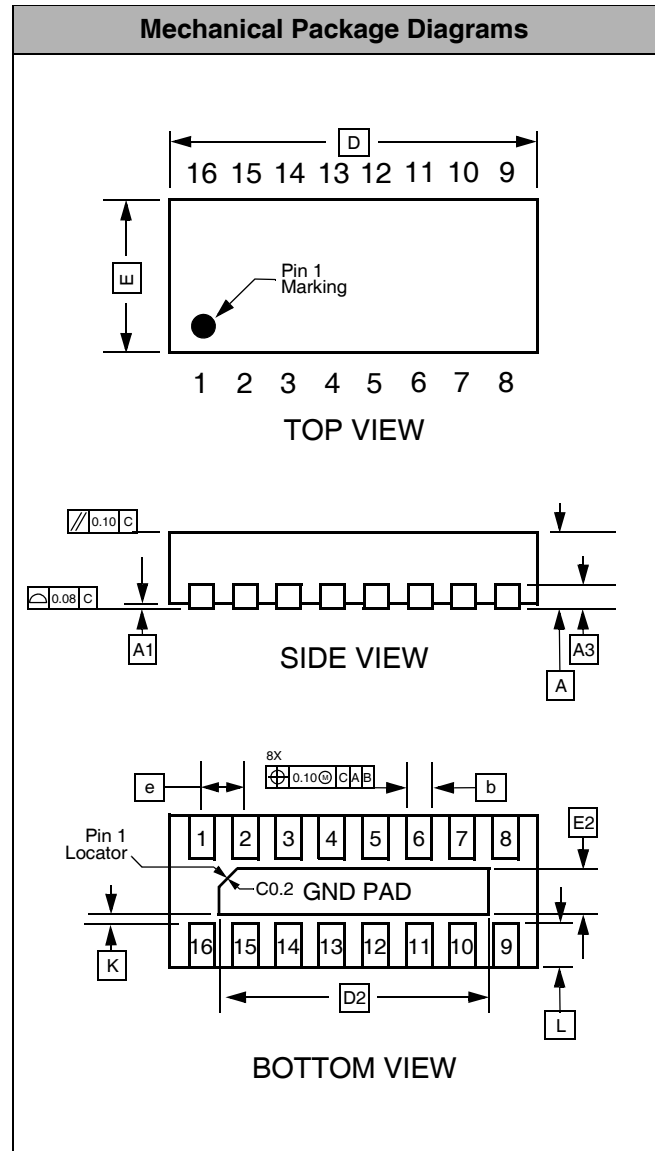
Dimensions for 16-Lead, 0.4mm pitch TDFN package
