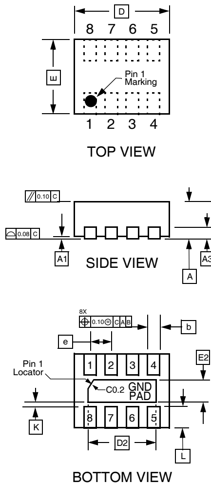
Dimensions for 8-Lead, 0.4mm pitch TDFN package
