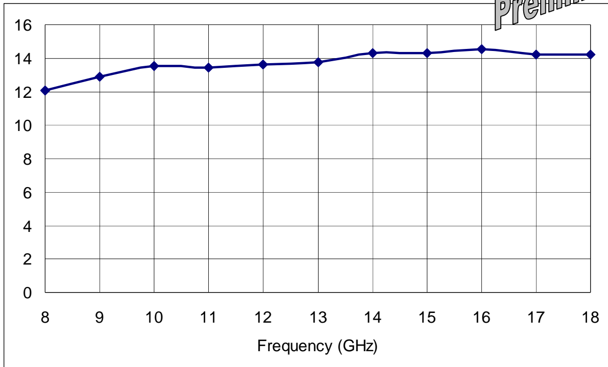
Output power @ 1dB compression (dBm)
