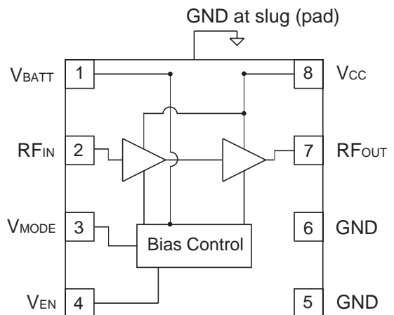
Figure 1: Block Diagram
