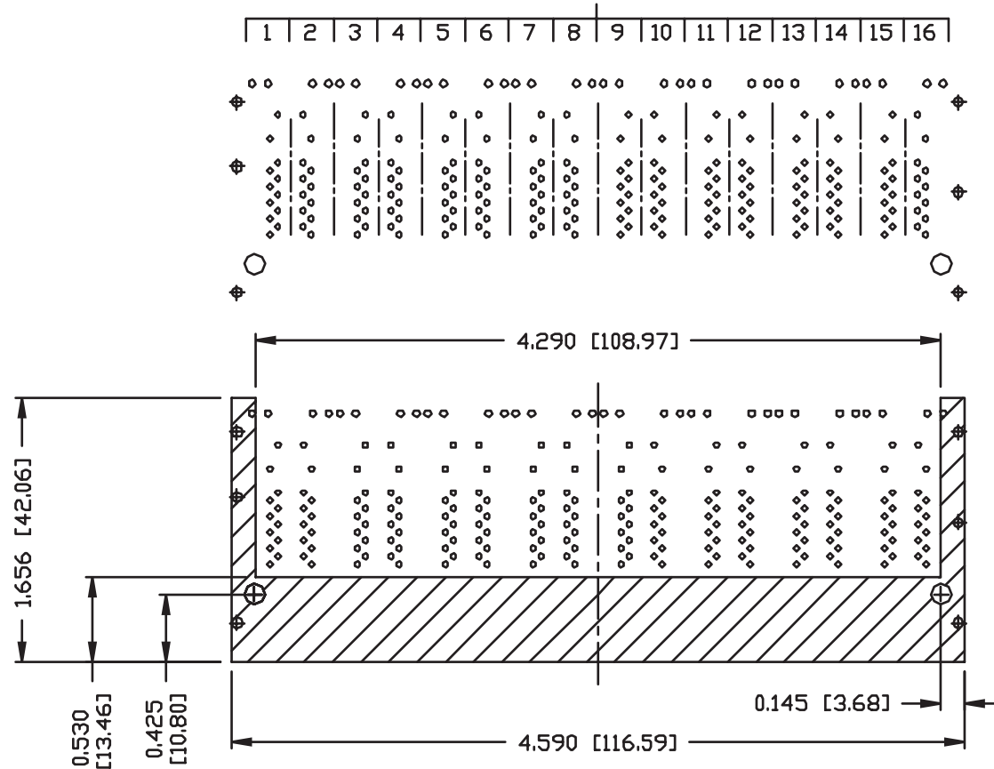
PORT ASSIGNMENT (COMPONENT SIDE VIEW)
