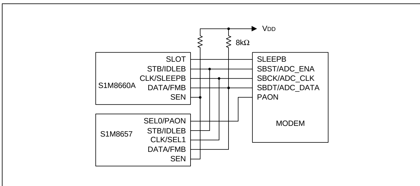
Figure 12. Serial Bus connection
