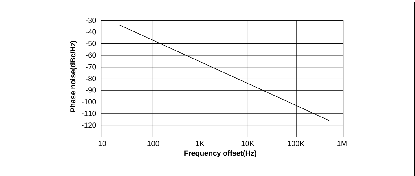
Figure 17. S1M8660A IF VCO Open Loop Phase Noise
