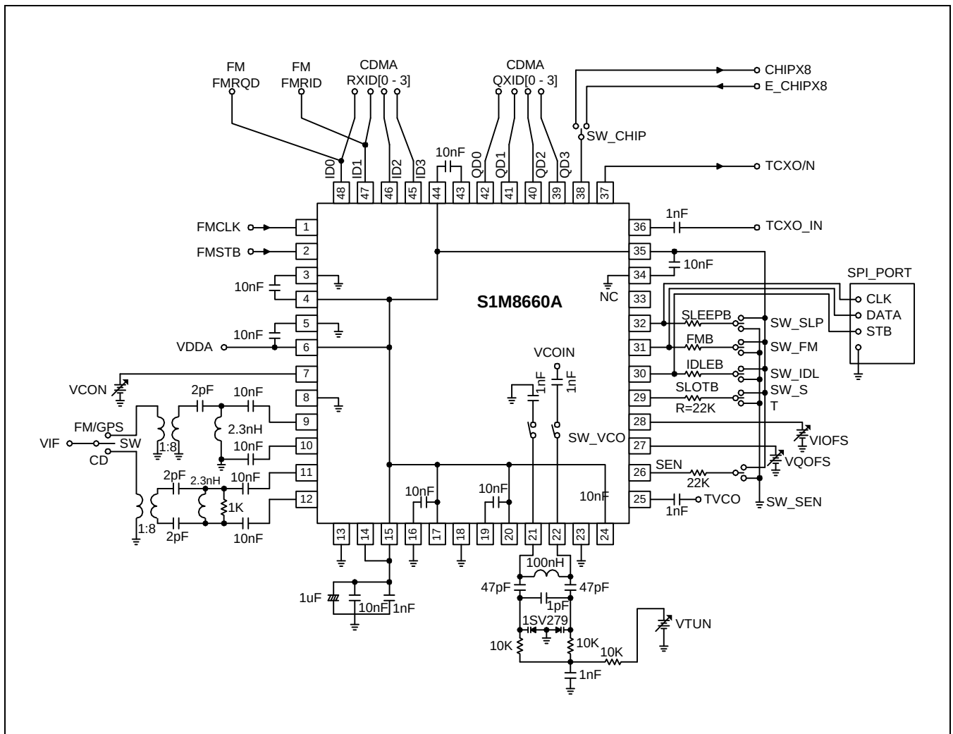
Figure 24. Test Circuit
