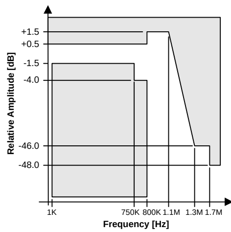
Figure 10. GPS Rx Low Pass Filter Mask
