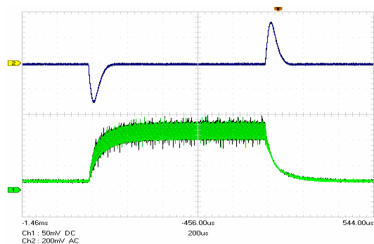
FIG. 8 Supply current through transient event (0.5-4A) Current scale is 0.5A per division
