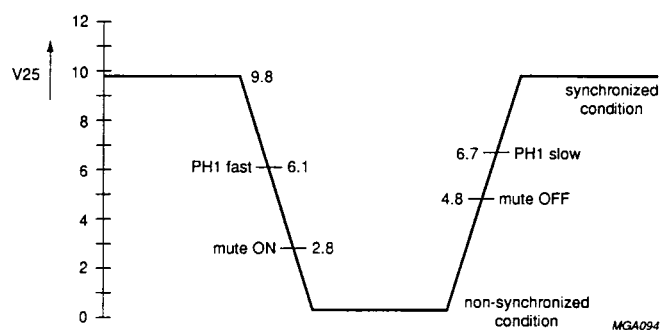
Fig.7 Switching levels coincidence detector.
