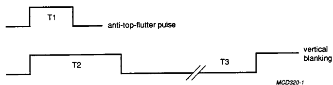
Fig.8 Anti-top-flutter pulse.
