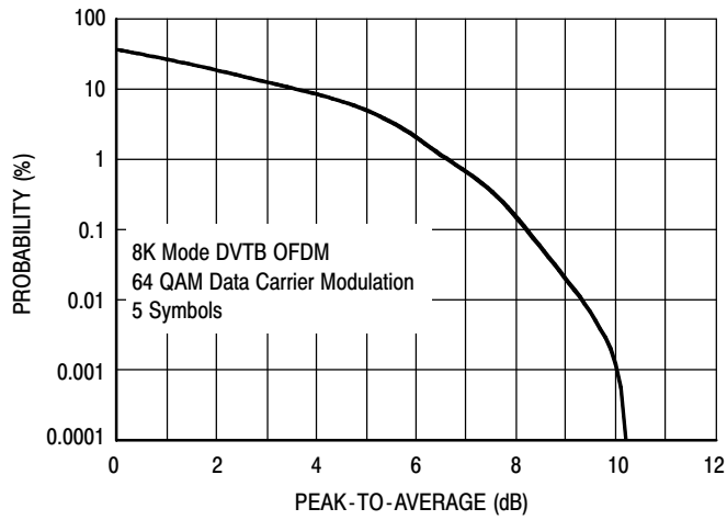
Figure 14. Single-Carrier DVB OFDM
