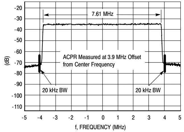
Figure 15. 8K Mode DVB OFDM Spectrum
