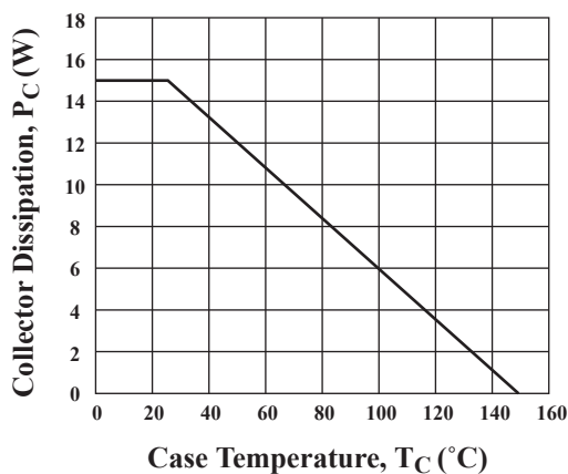
FIG.10 P_C - T_C
