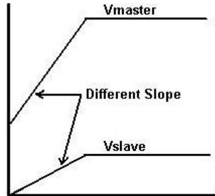
Figure 10. Ratiometric Tracking
