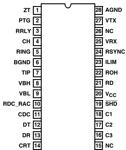
HC55142 (28 LEAD SOIC) TOP VIEW
