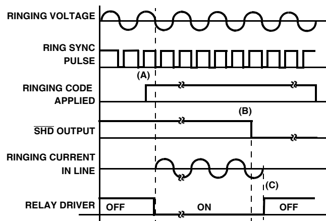
FIGURE 19. RINGING SEQUENCE
