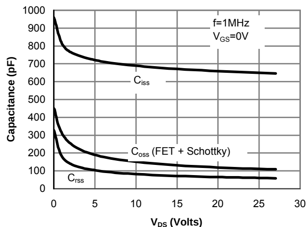
Figure 8: Capacitance Characteristics: MOSFET + Parallel Schottky
