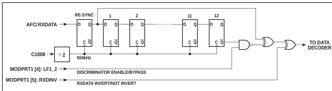
Fig. 21 Modern discriminator
