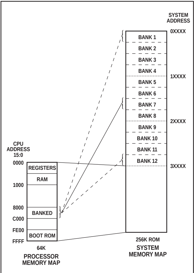
Fig. 15 Memory Map and Banked Addressing
