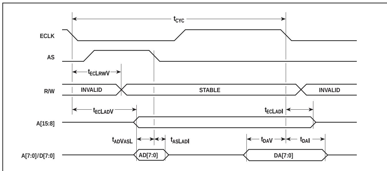
Fig.6 ACE9050 6303 Emulation mode Read/Write cycles timing diagram
