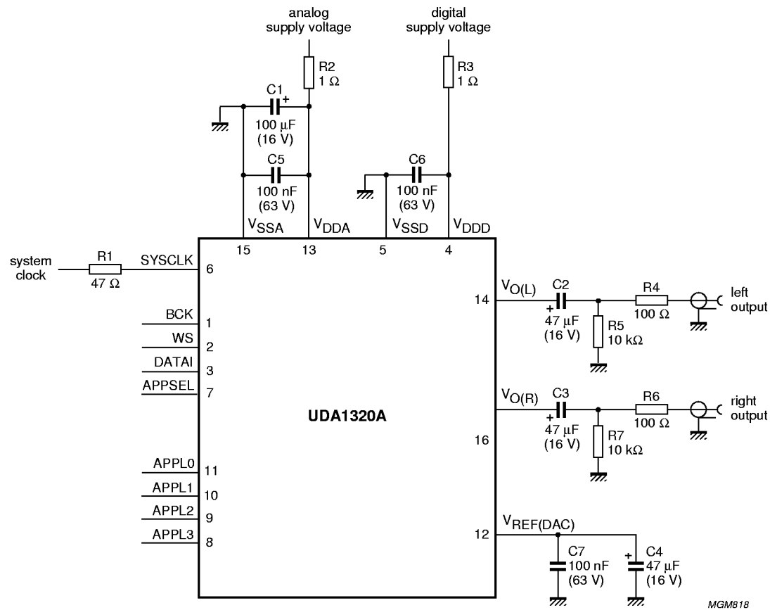
Fig.8 Application schematic.
