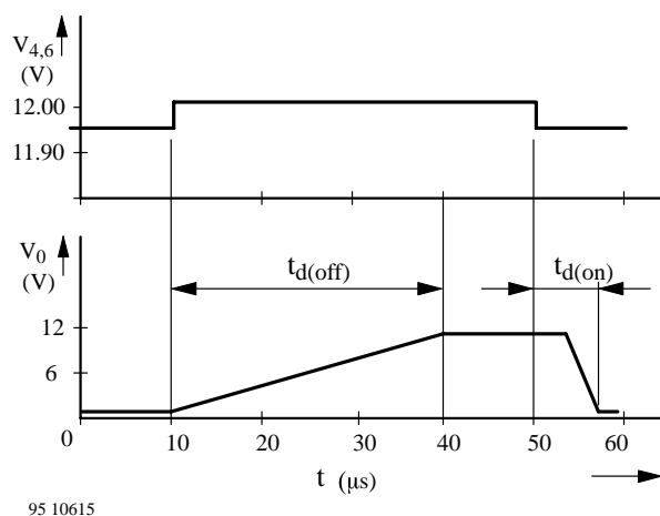
Figure 2. Timing diagram
