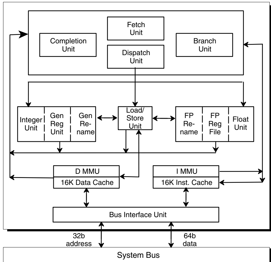
Figure 1. Block Diagram
