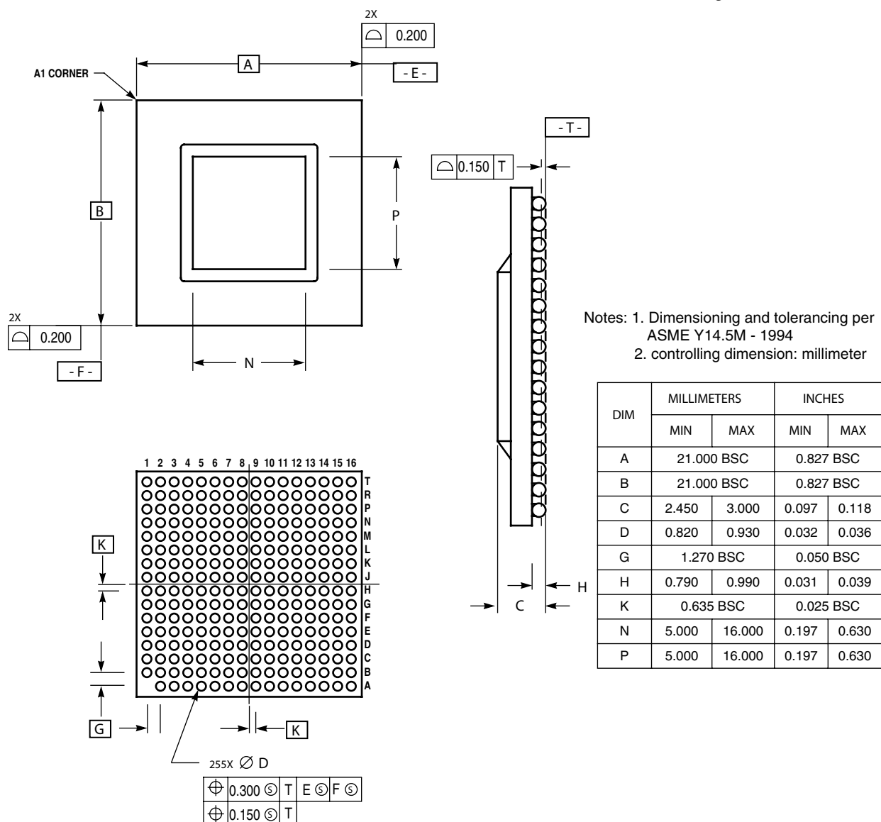
Figure 15. Mechanical Dimensions and Bottom Surface Nomenclature of the CBGA Package
