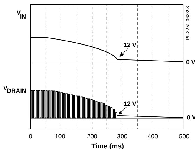
Figure 8. TinySwitch Power Down Timing Diagram.
