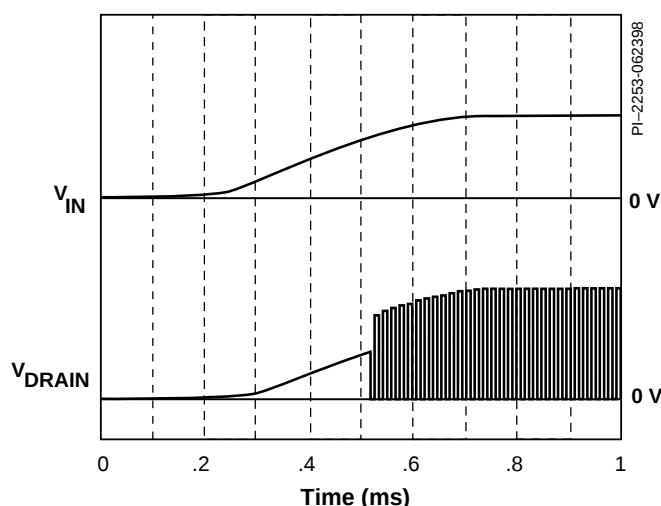
Figure 7. TinySwitch Power-Up Timing Diagram.
