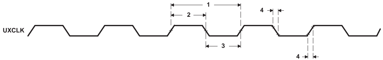
Figure 56. UXCLK Timing
