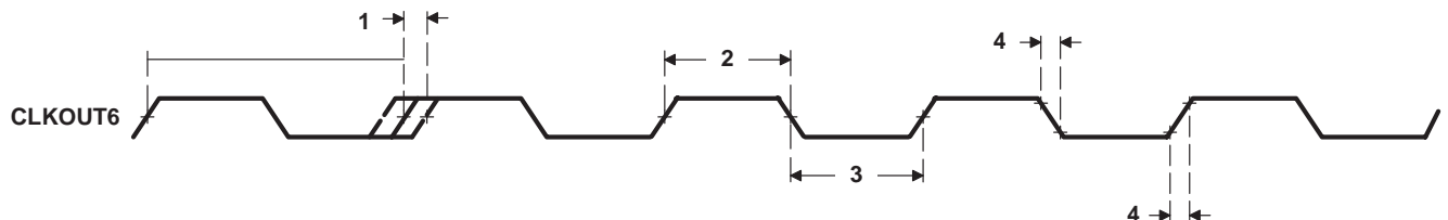
Figure 17. CLKOUT6 Timing
