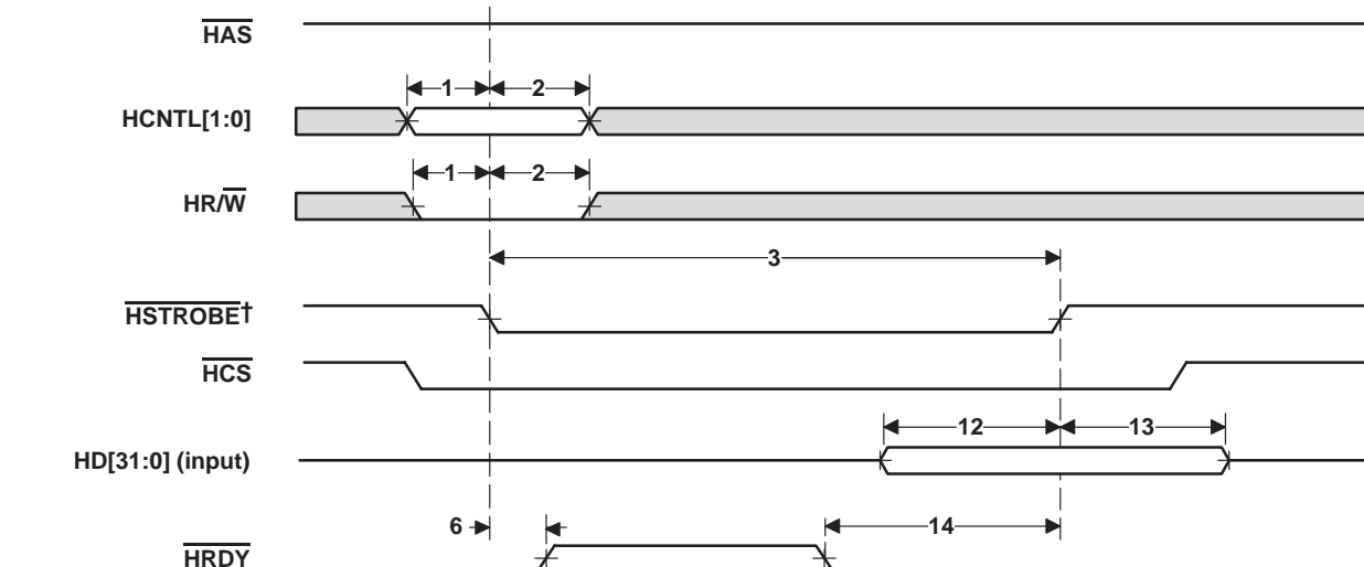
Figure 44. HPI32 Write Timing ( \overline{\text{HAS}} Not Used, Tied High)
