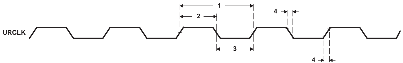
Figure 57. URCLK Timing
