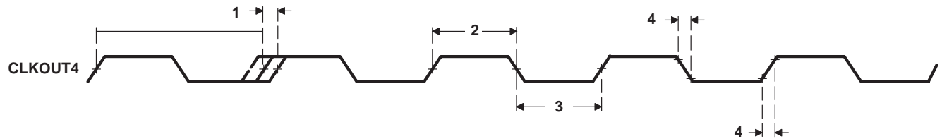
Figure 16. CLKOUT4 Timing
