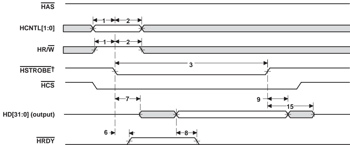
Figure 42. HPI32 Read Timing ( \overline{HAS} Not Used, Tied High)
