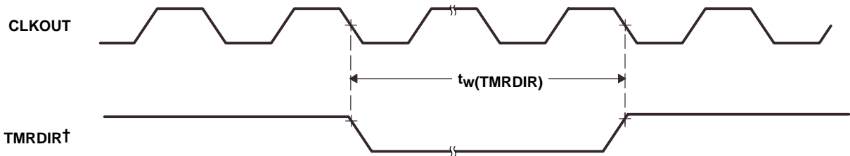
Figure 30. Capture/TMRDIR Timing
