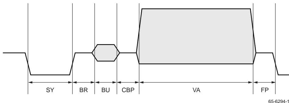
Figure 9. Horizontal Timing
