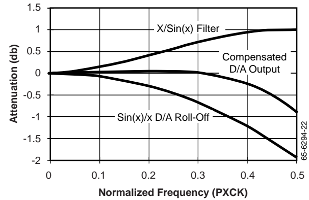
Figure 20. X/SIN(X) Filter
