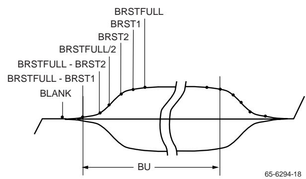
Figure 16. Burst Envelope
