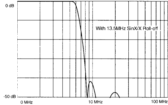
Figure 34. Stop Band
