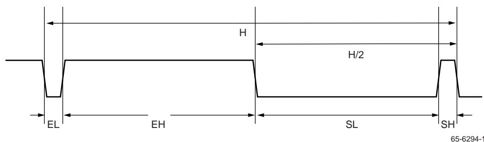
Figure 10. Horizontal Timing – Vertical Blanking
