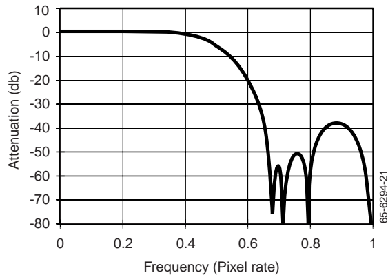
Figure 18. Interpolation Filter
