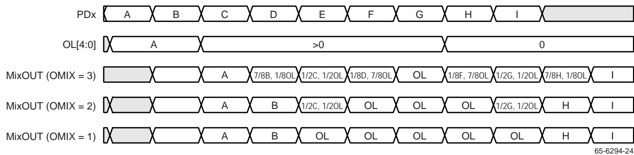
Figure 22. Overlay Outputs
