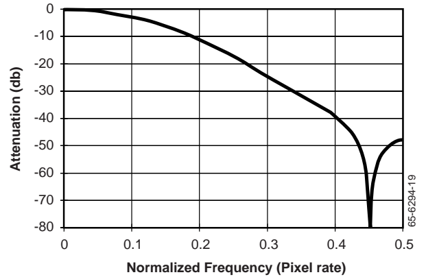
Figure 17. Gaussian Filter Response
