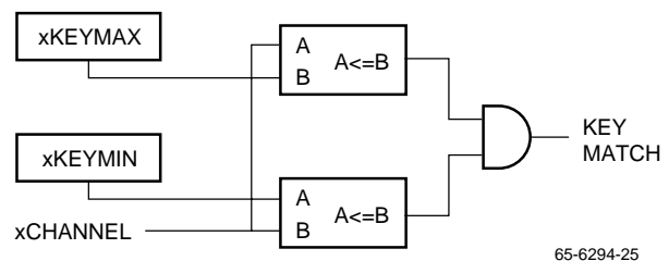
Figure 23. Data Keying
