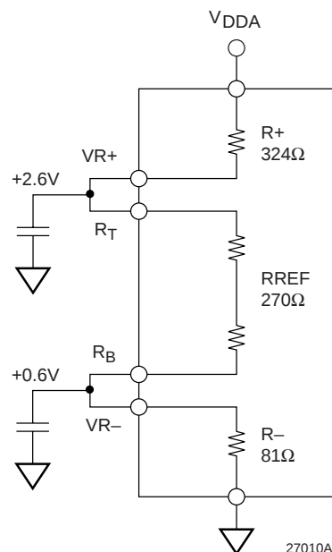
Figure 1. Reference Resistors
