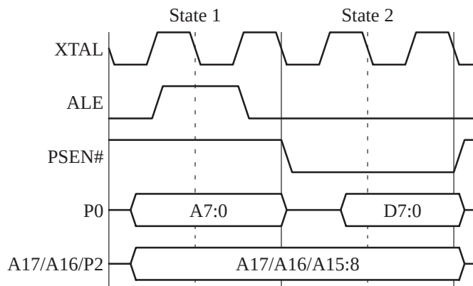
Figure 3.2 External Code Fetch (Non-Page Mode)
