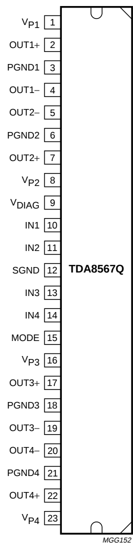
Fig.2 Pin configuration.
