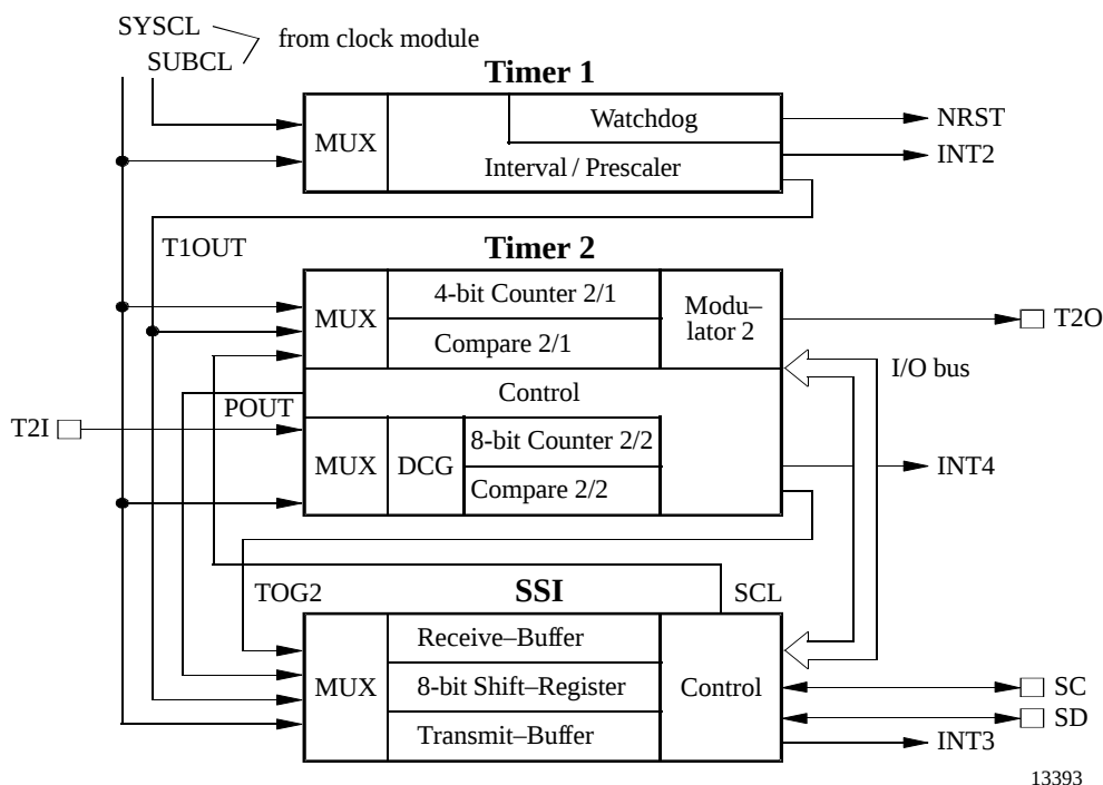
Figure 26. UTCM block diagram
