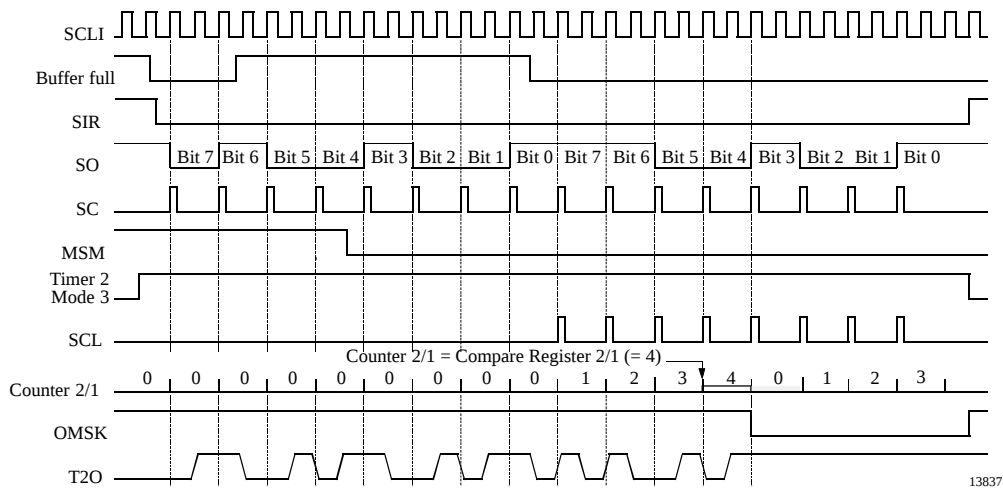
Figure 56. Manchester modulation 2
