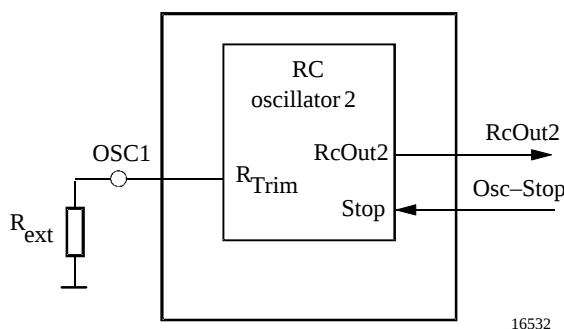
Figure 17. RC-oscillator 2
