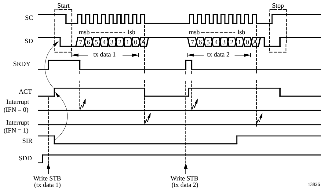
Figure 47. Example of I 2 C transmit dialog
