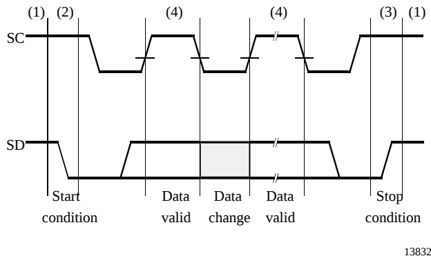
Figure 49. I 2 C bus protocol 1
