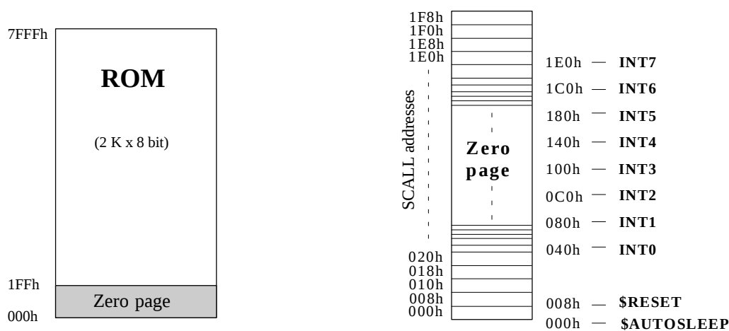
Figure 4. ROM map of T44C080
