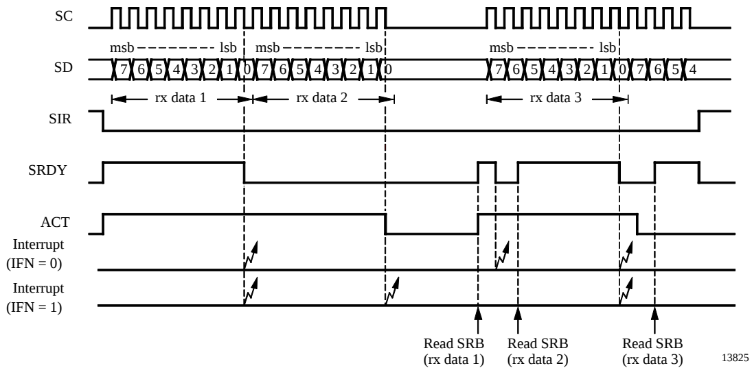
Figure 46. Example of 8-bit synchronous receive operation
