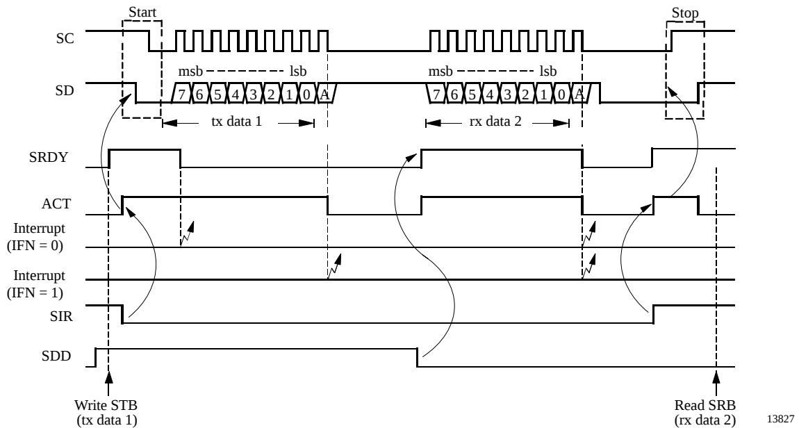
Figure 48. Example of I 2 C receive dialog
