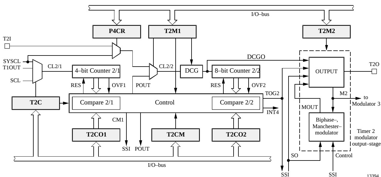
Figure 29. Timer 2
