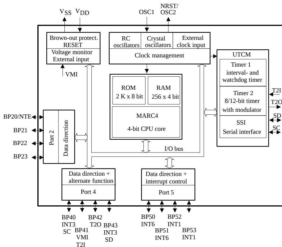
Figure 1. Block diagram of the T44C080
