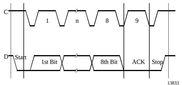
Figure 50. I 2 C bus protocol 2
