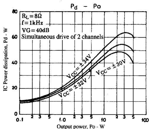
Figure 1. STK4172II Pd - Po ( R_l = 8\Omega )
