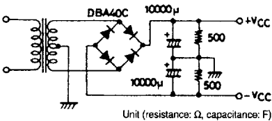
Specified Transformer Power Supply (Equivalent to MG-200)
