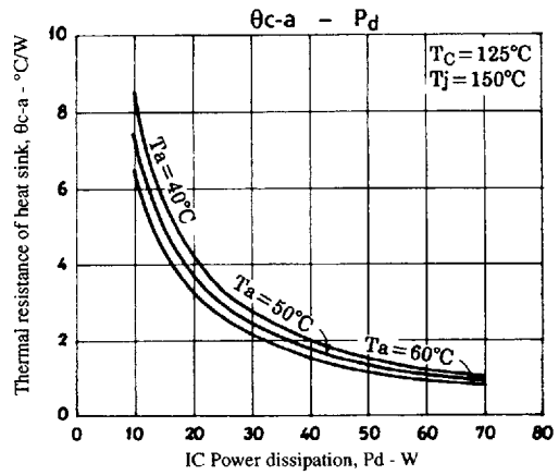
Figure 3. STK4172II θc-a - Pd
