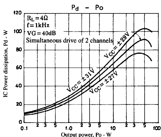
Figure 2. STK4172II Pd - Po ( R_i = 4\Omega )
