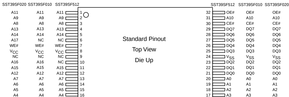
FIGURE 1: PIN ASSIGNMENTS FOR 32-PIN TSOP (8mm x 14mm)
