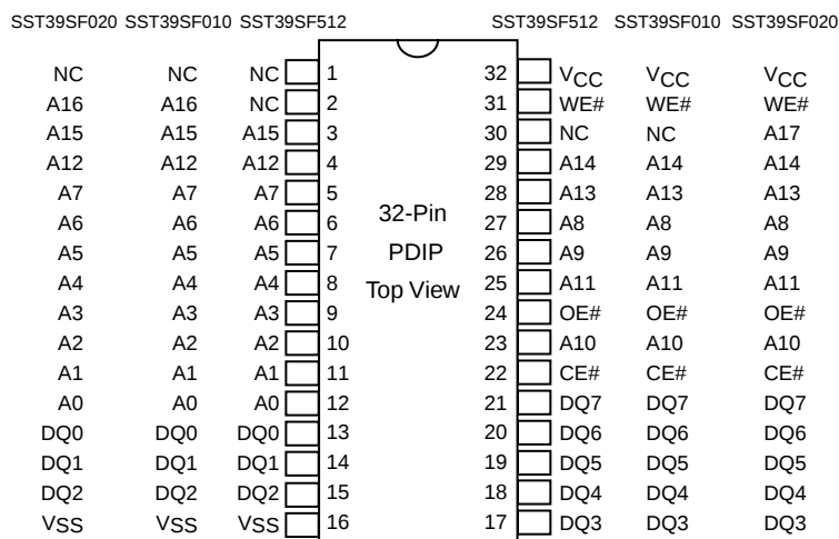
FIGURE 2: PIN ASSIGNMENTS FOR 32-PIN PDIP
