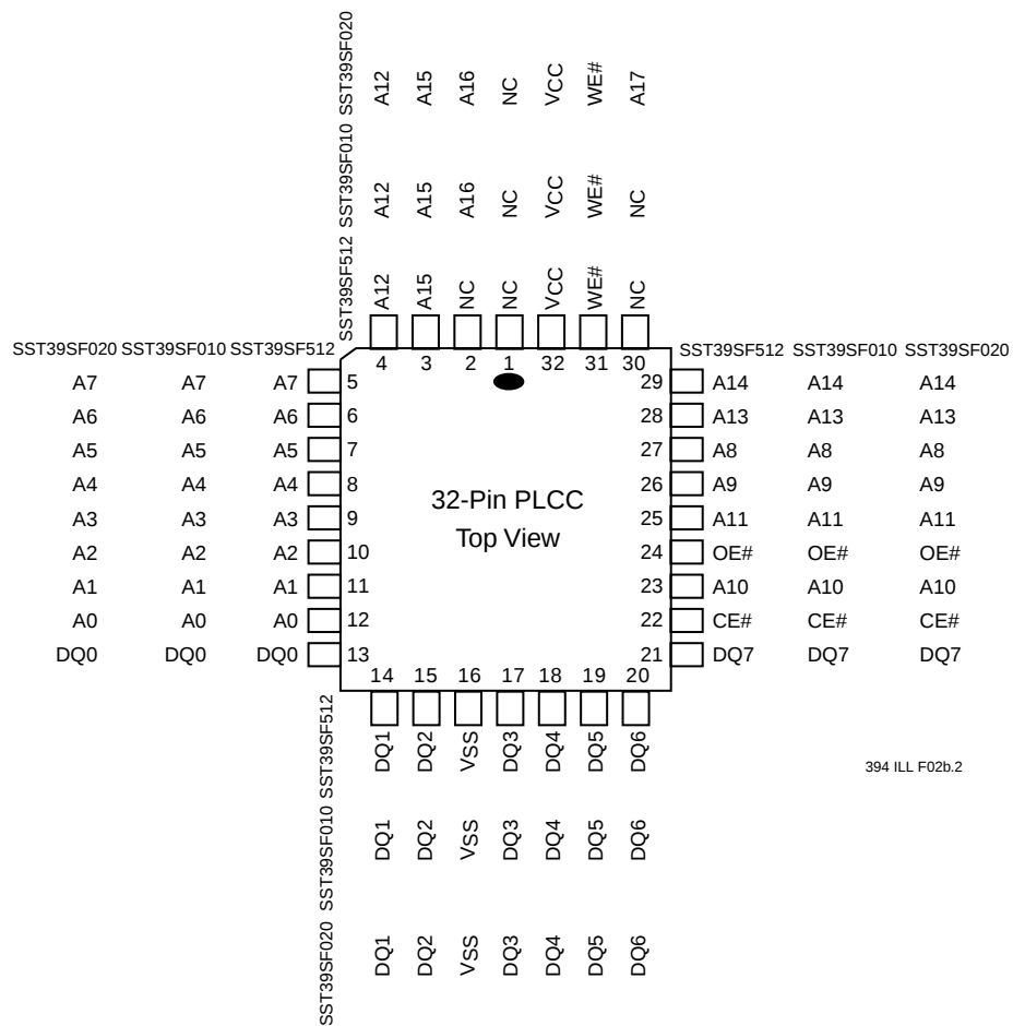
FIGURE 3: PIN ASSIGNMENTS FOR 32-PIN PLCC
