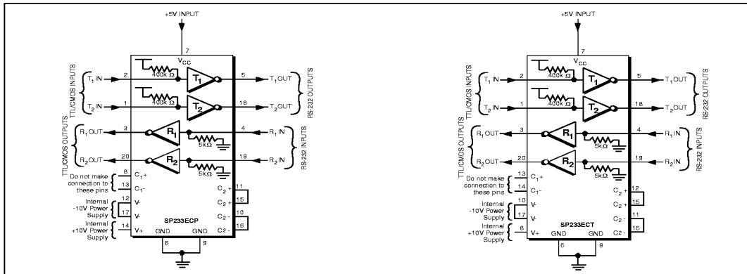
Figure 2. Typical Circuits using the SP233ECP and SP233ECT
