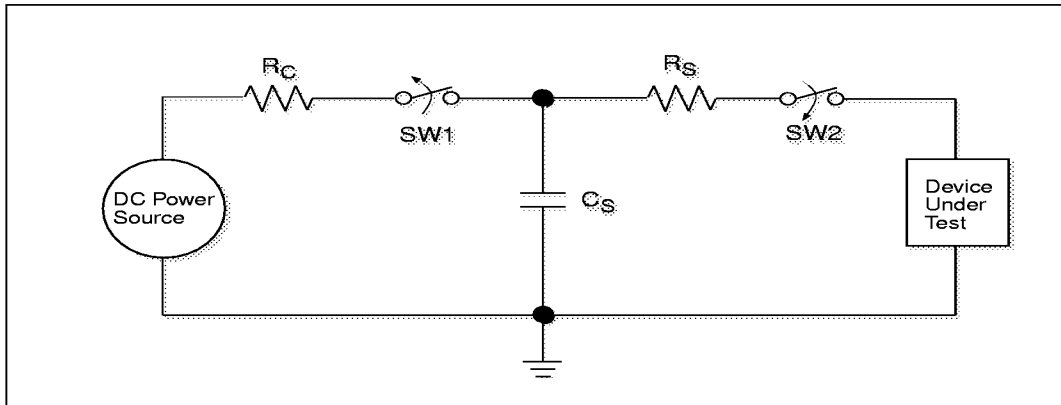
Figure 9. ESD Test Circuit for Human Body Model
