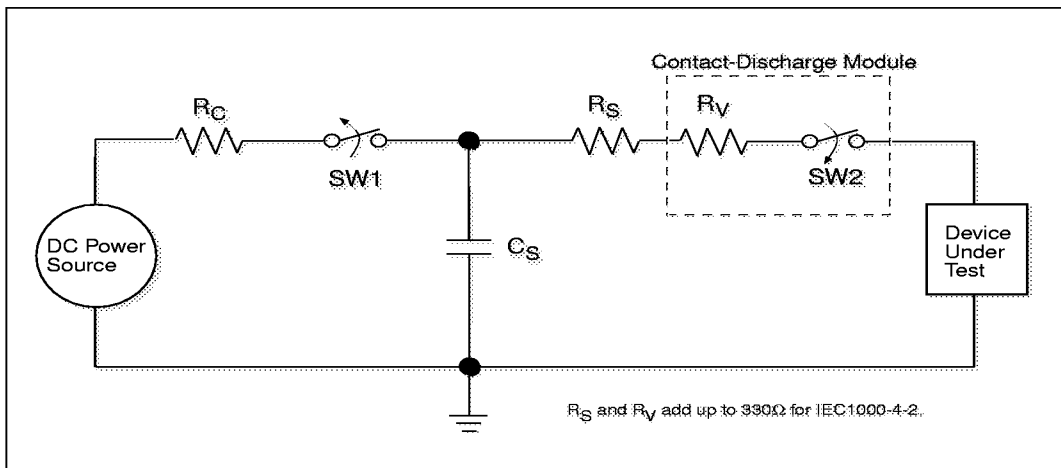
Figure 10. ESD Test Circuit for IEC1000-4-2
