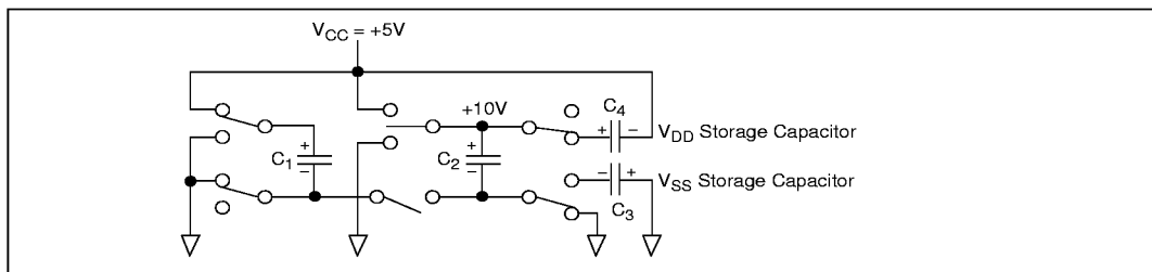
Figure 8. Charge Pump — Phase 4
