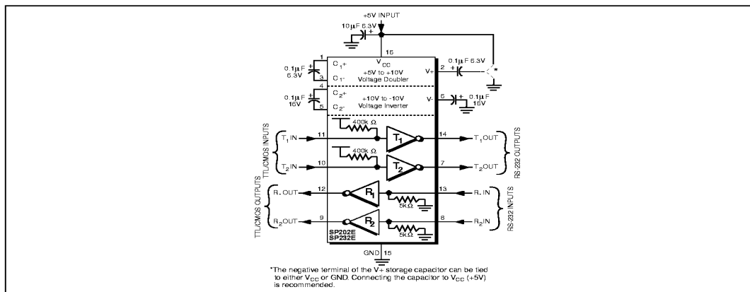
Figure 1. Typical Circuit using the SP202E or SP232E.
