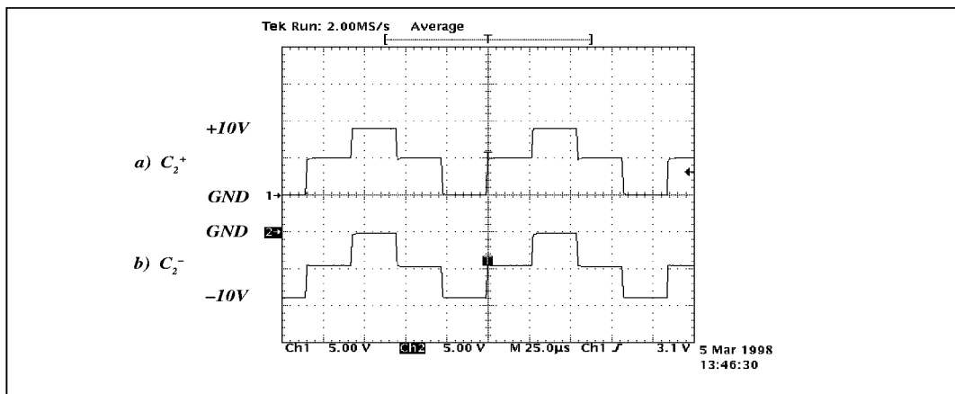
Figure 6. Charge Pump Waveforms
