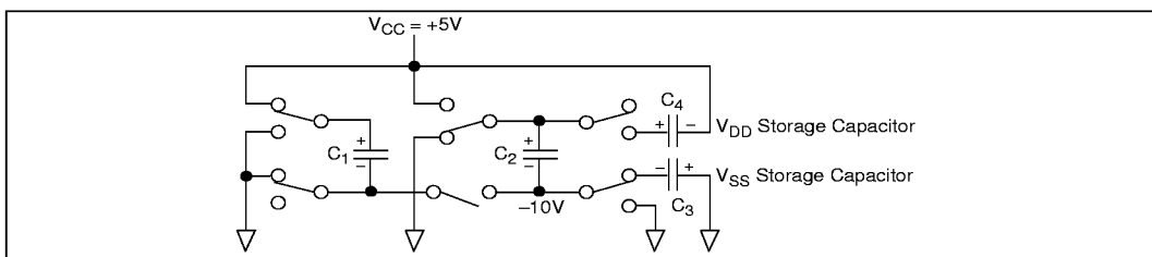
Figure 5. Charge Pump — Phase 2
