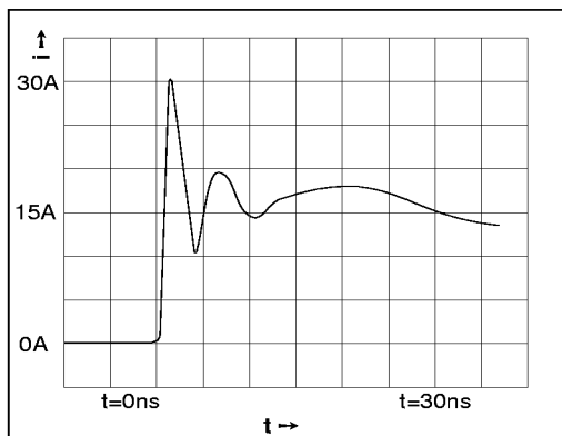
Figure 11. ESD Test Waveform for IEC1000-4-2
