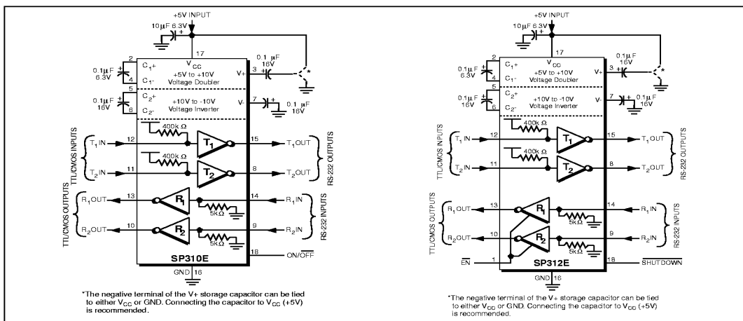
Figure 3. Typical Circuits using the SP310E and SP312E
