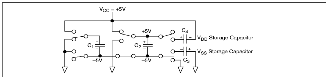
Figure 7. Charge Pump — Phase 3
