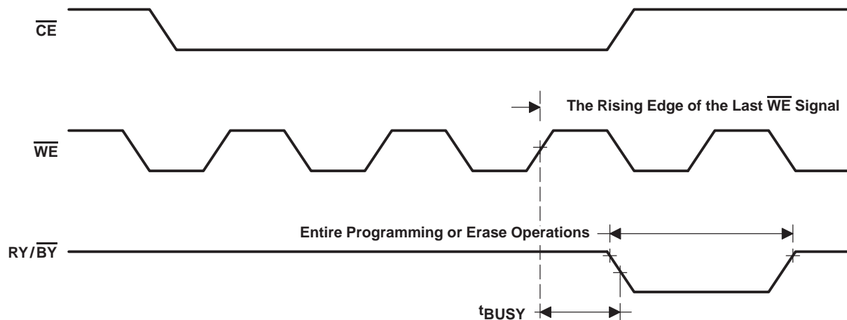
Figure 24. \text{RY}/\overline{\text{BY}} Timing Diagram During Program/Erase Operations
