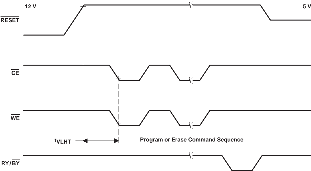
Figure 23. Temporary Sector-Unprotect Timing Diagram
