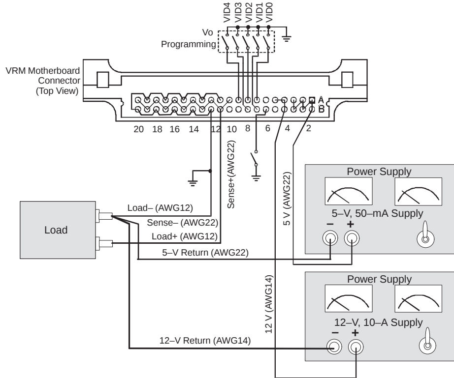
Figure 3–4. Input/Output Connections
