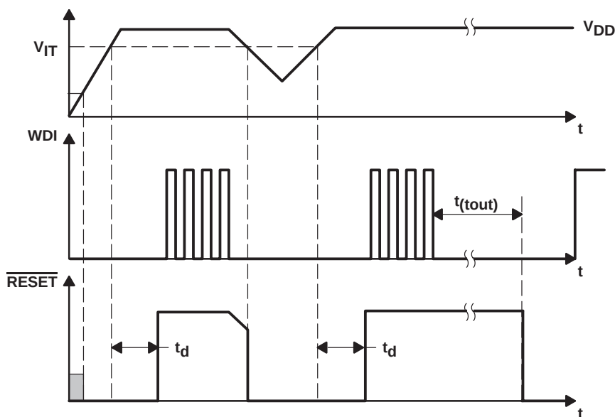
Figure 1. Watchdog Timing
