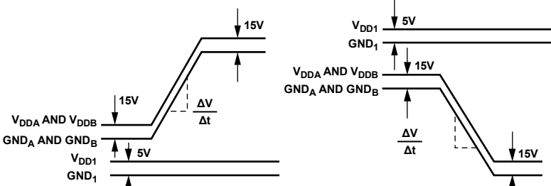
Figure 11. Common-Mode Transient Immunity Waveforms—Input to Output
