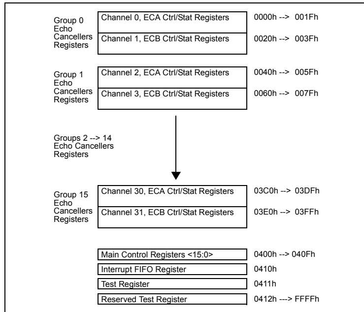
Figure 10 - Memory Mapping
