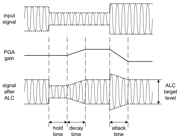
Figure 21 ALC Operation
