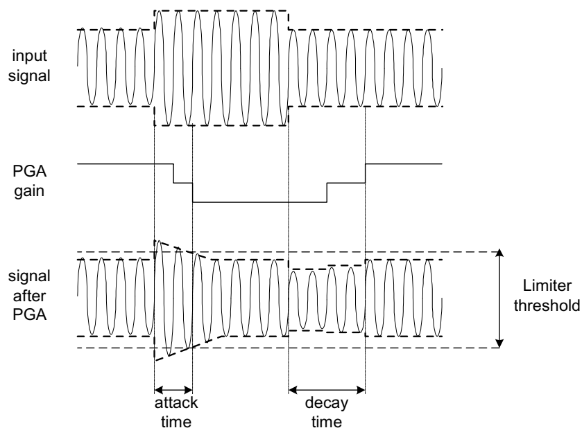
Figure 20 Limiter Operation
