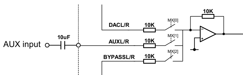
Figure 38 5.1 Channel Input Multiplexor Configuration
