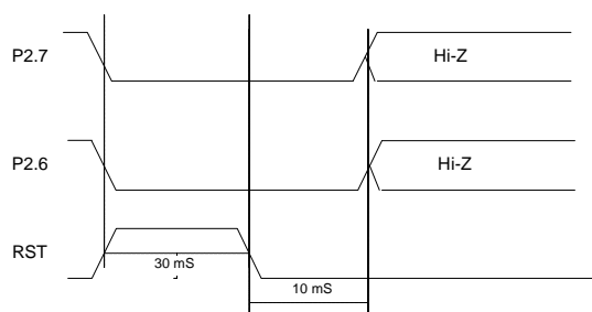
The Reset Timing For Entering F04KBOOT Mode
