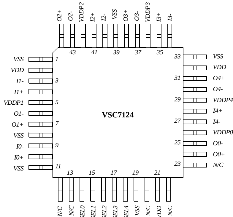
Figure 3: Pin Diagram
