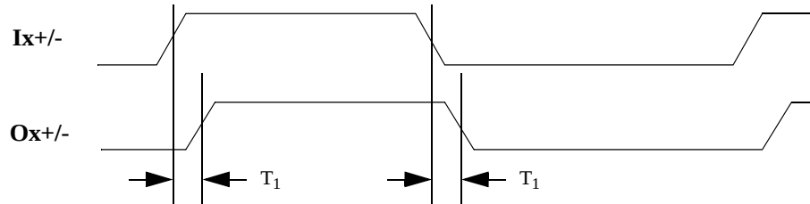
Figure 2: Timing Waveforms
