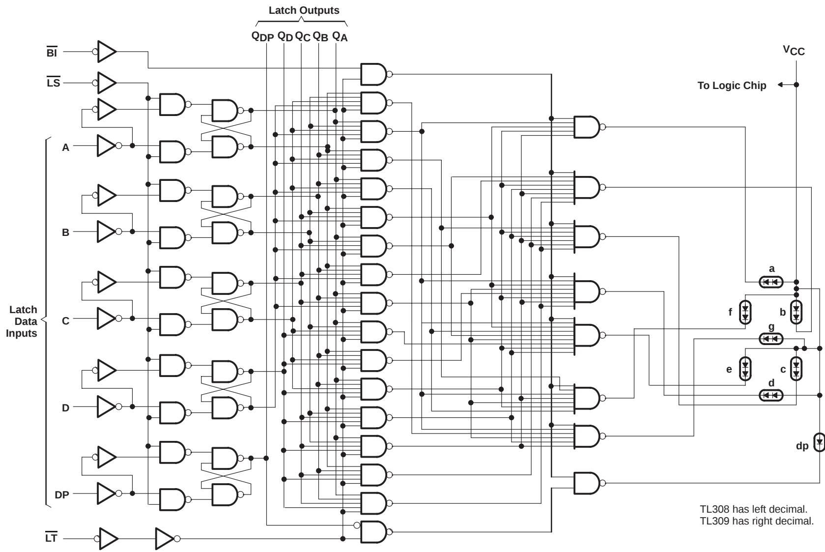
logic diagram
