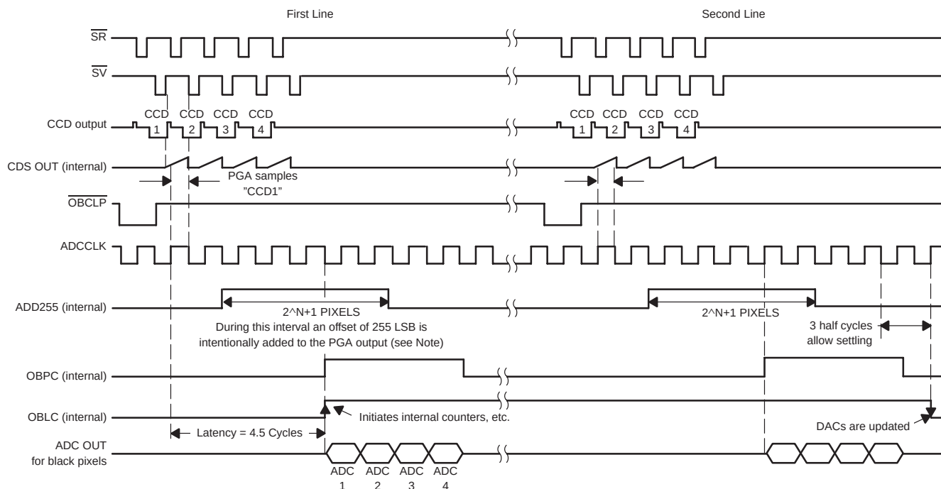
Figure 6. Optical Black and Offset Correction Timing
