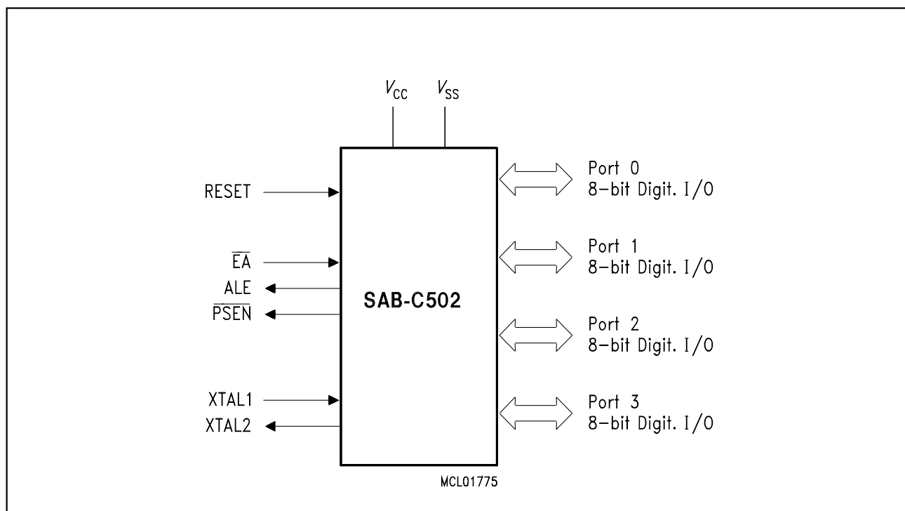
Logic Symbol
