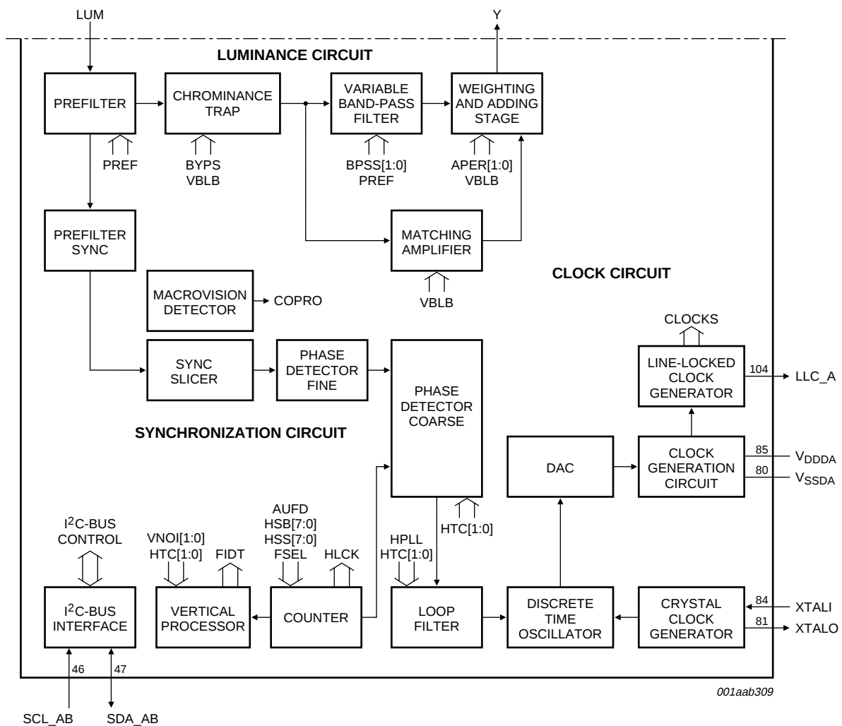
Fig 17. Luminance and sync processing (continued from Figure 10).
