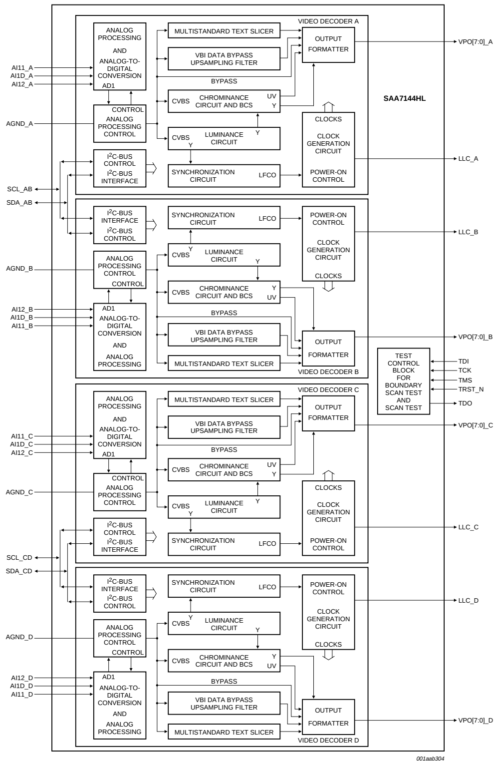
Fig 1. Block diagram of SAA7144HL.
